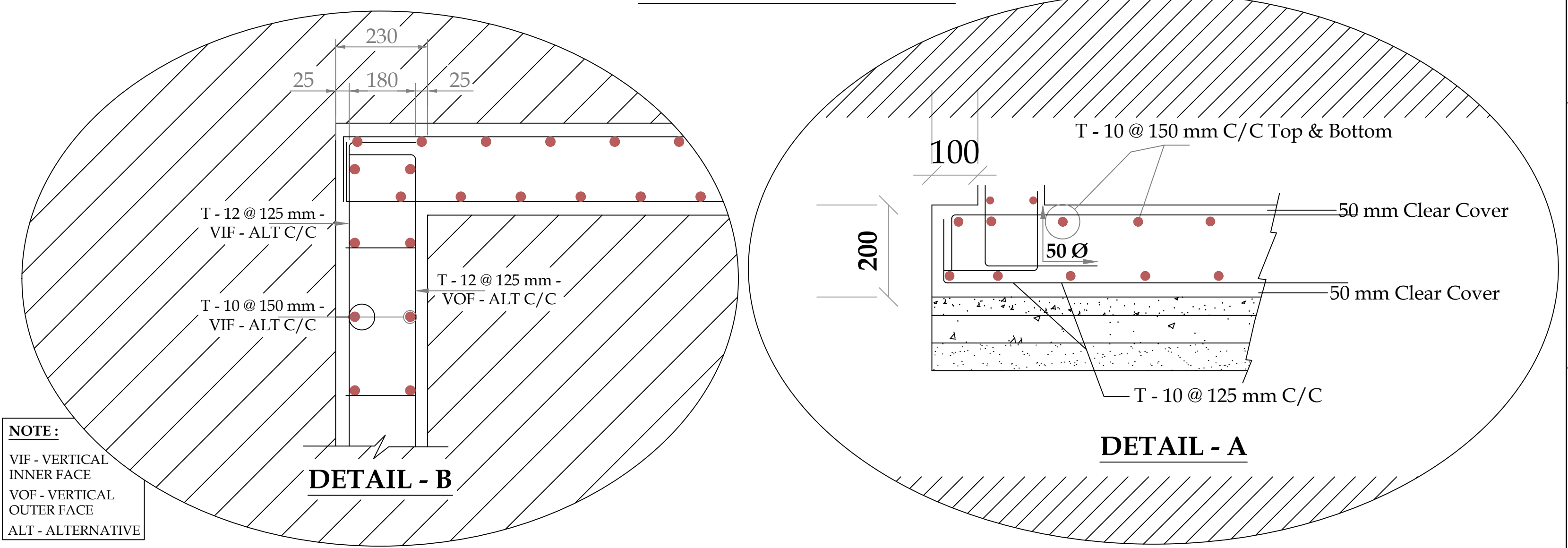
R.C.C CULVERT SLAB DETAIL
