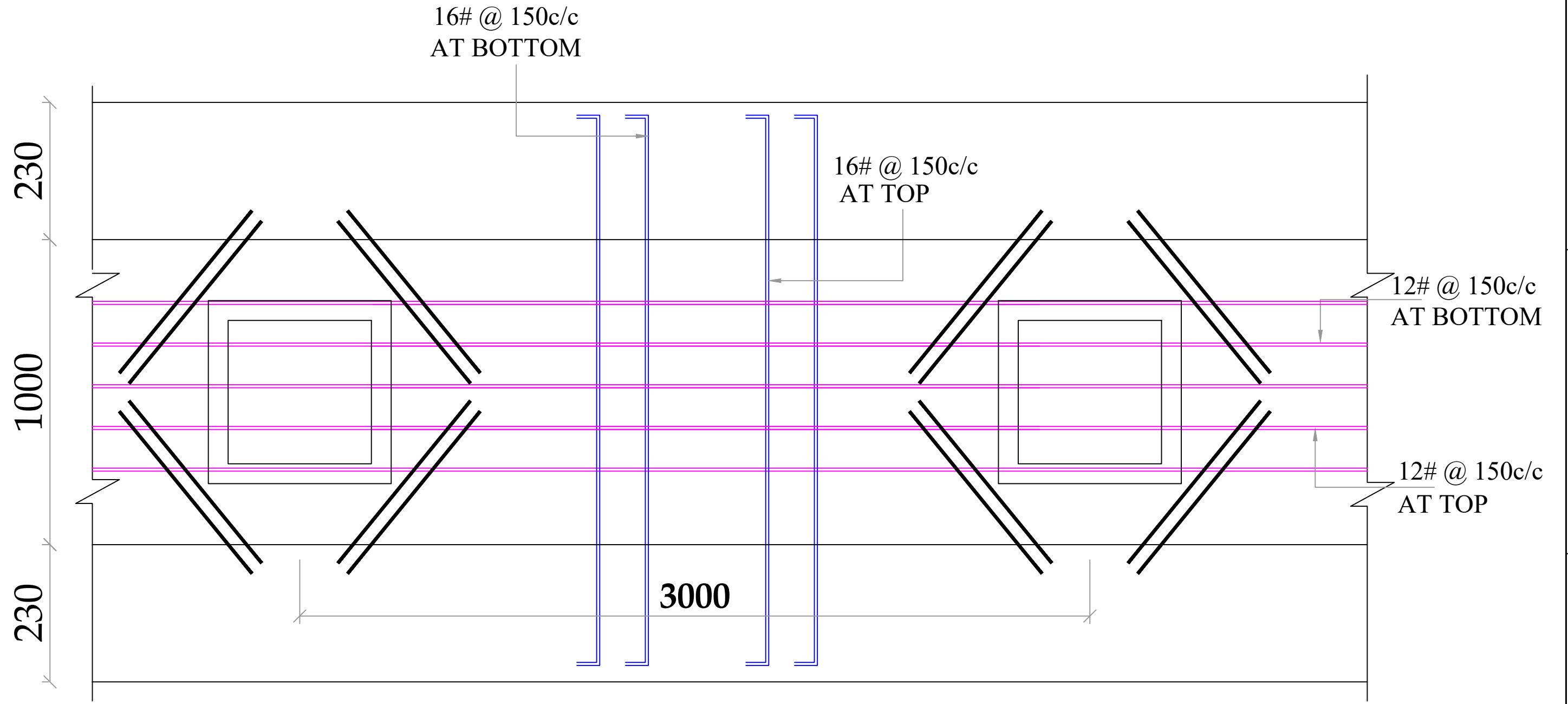
R.C.C CULVERT SLAB DETAIL
